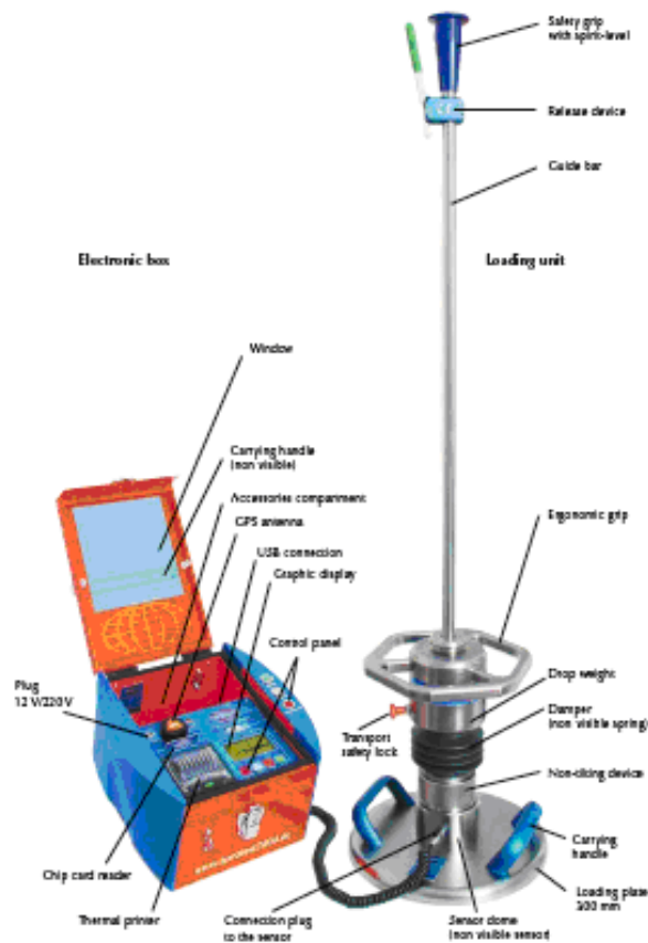
Figura 3. Light Weight Deflectometer
